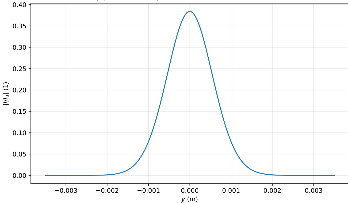
Intensity profile I(x = 0, y, z = 2.946)/I_0 , P_{in}=0.2P_{cr} , artificial time
